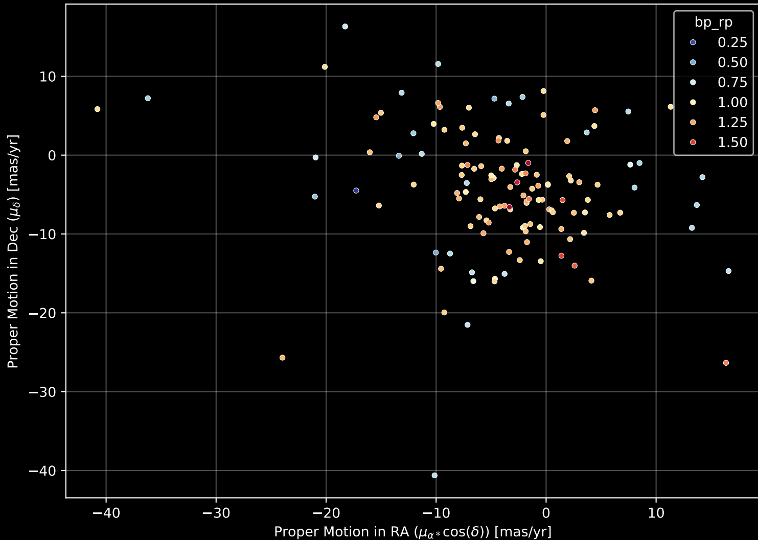
APOGEE DR17 Field: [046+48] Proper Motion Diagram (n= 131)
