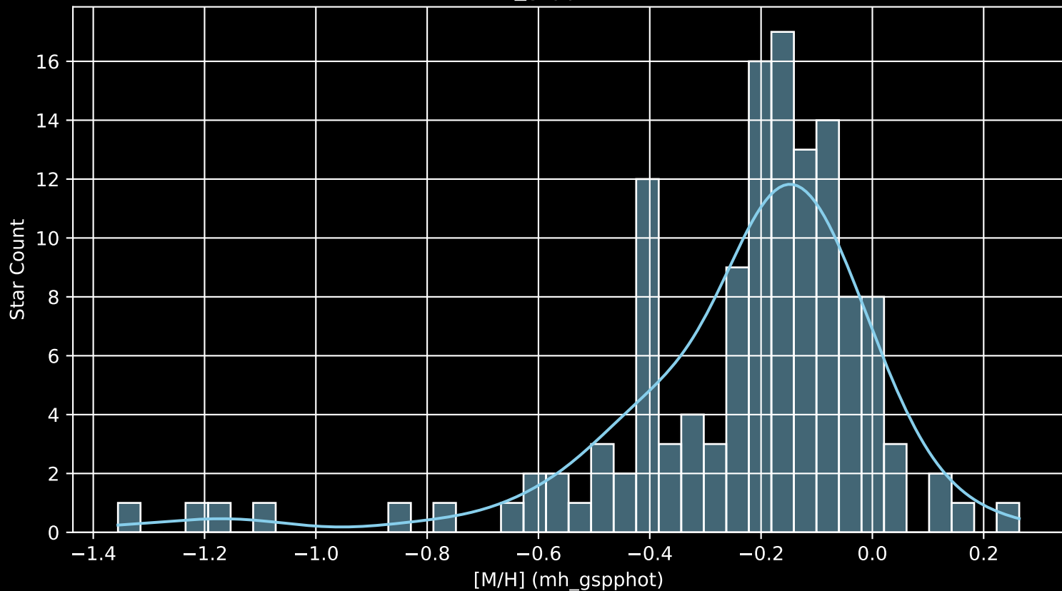
APOGEE DR17 Field: [046+48 [M/H] (mh_gspphot) (n= 131)
