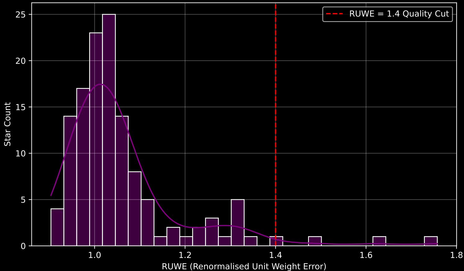
GAPOGEE DR17 Field [046+48] RUWE Distribution (n= 130)
