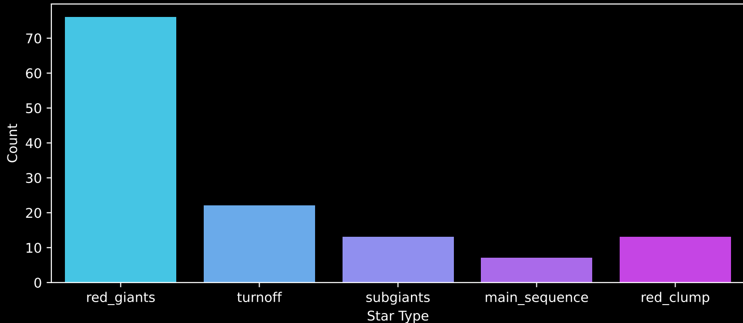
APOGEE DR17 Field: [046+48] Count plot of Star Type
