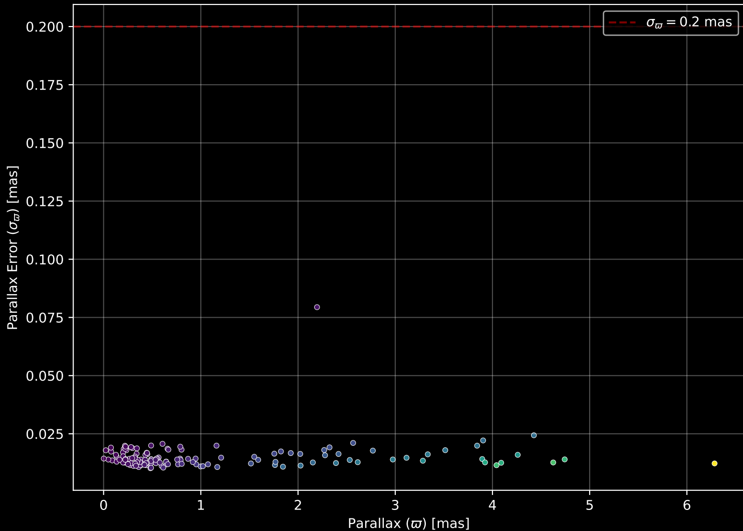
APOGEE DR17 Field: [046+48] Parallax Quality (n= 131)
